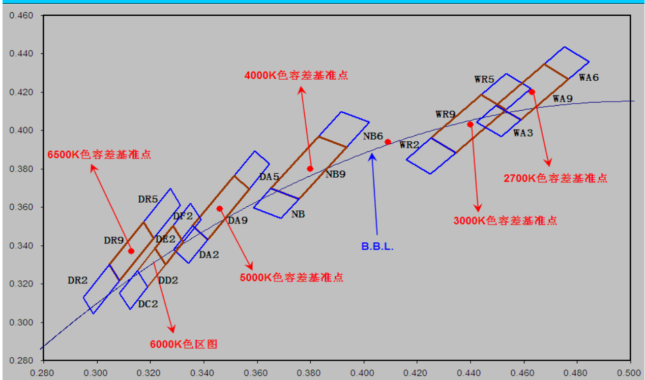
TOP LED 色区汇总图(大BIN色区)
